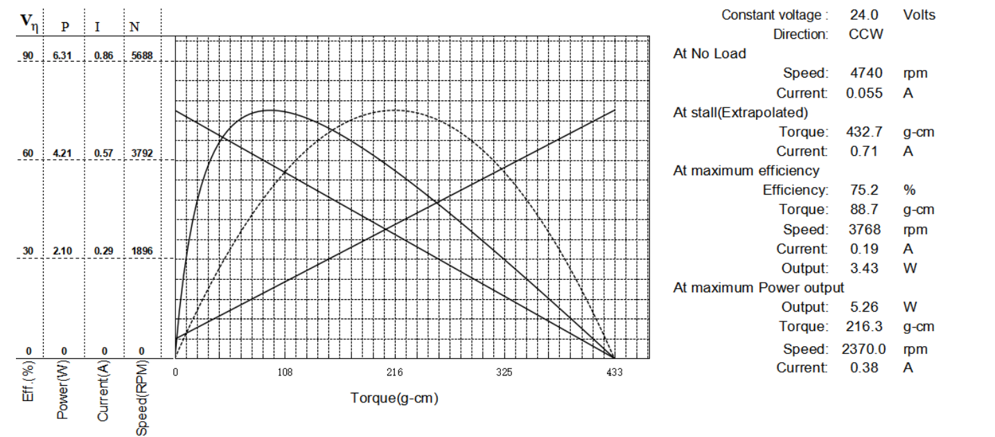
电机曲线图/Motor Characteristic Curves
